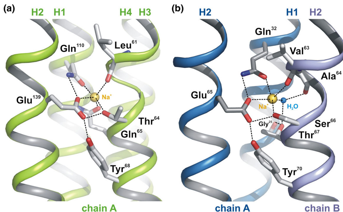
Fig. 3. Na + binding in the rotor rings of the V-ATPase from E. hirae and the F-ATP synthase from I. tartaricus . (a) In the K 10 -ring from E. hirae (PDB ID code 2b12), 12 Na + is coordinated within a single K-subunit, each of which comprises four α-helices (H1–H4; green). (b) In the c 11 -ring from I. tartaricus , 8 the Na + binding site is located in between the inner (H2; blue) and the outer (H1; blue) helices of one c-subunit, and the outer helix (H2; purple) of the adjacent c-subunit. Dashed lines indicate ion-coordination contacts and the network of hydrogen bonds at the site.
