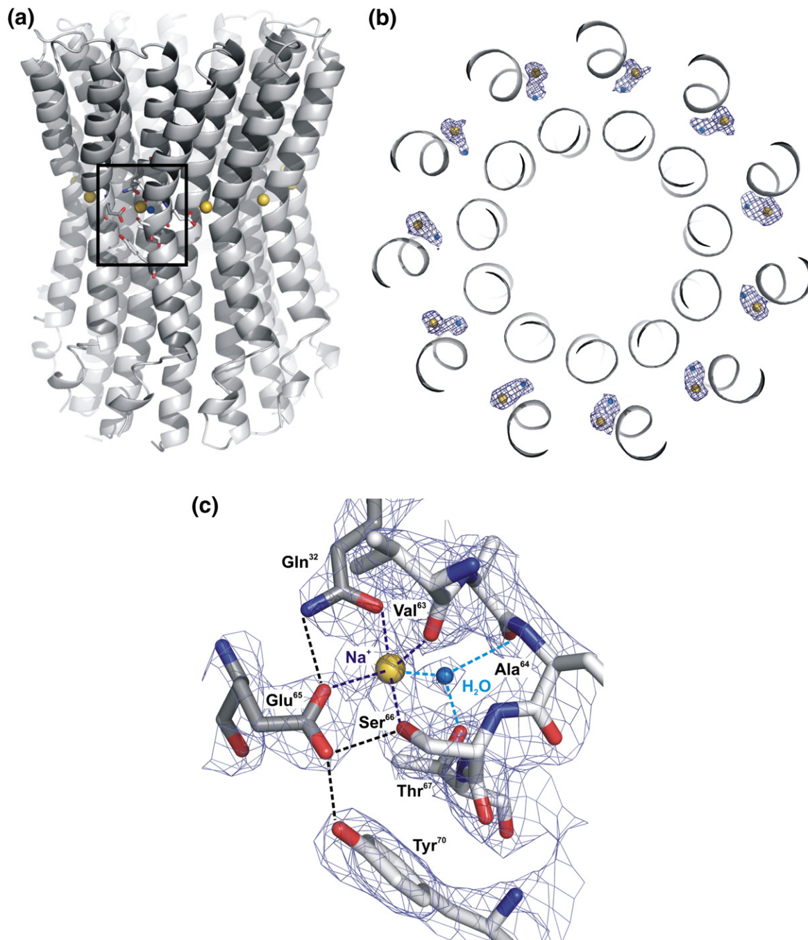
Fig. 1. The Na + binding site in the c 11 -ring from I. tartaricus ATP synthase. (a) The ring is composed of 11 c-subunits, each comprising two transmembrane helices shown as gray ribbons. The binding sites for Na + (yellow spheres) are located in between adjacent subunits. (b) Nonsymmetrized electron density peaks ( 2F_{\text{obs}} - F_{\text{calc}} map at 1.8\sigma ) corresponding to buried structural water molecules (blue spheres) that coordinate Na + (yellow spheres). The view is of a slice of density parallel with the plane of the membrane. (c) Close-up and electron density map of the Na + binding site ( 2F_{\text{obs}} - F_{\text{calc}} map at 1.8\sigma ) from the same viewpoint as the rectangle in (a). The amino acids involved in ion coordination are depicted in stick representation. Thr67 and Ala64 are also indicated (see Results). Ion-protein contacts and the network of hydrogen bonds in the site are indicated with broken lines.
